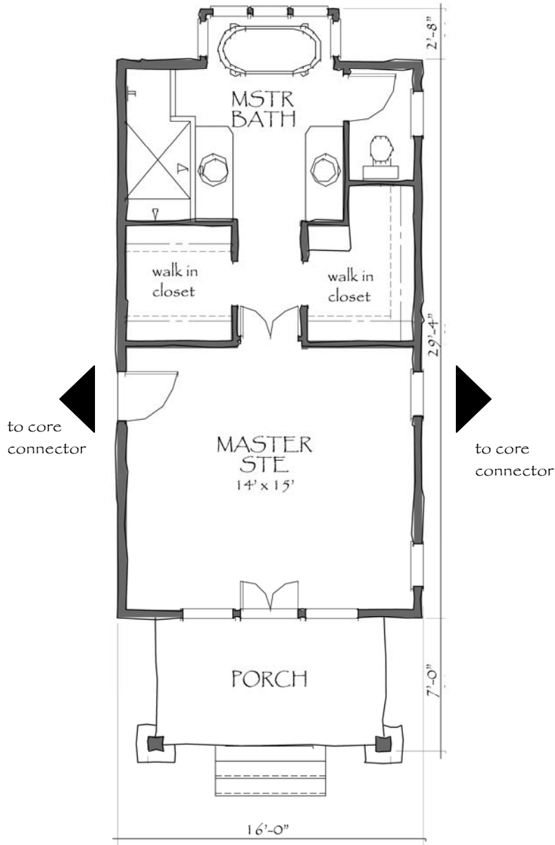
FLOOR PLAN
